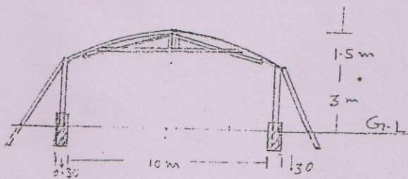
SECTIONAL ELEVATION AT X-X'
