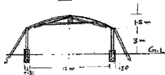
SECTIONAL ELEVATION AT X-X' DETAIL DRAWING OF NET HOUSE
